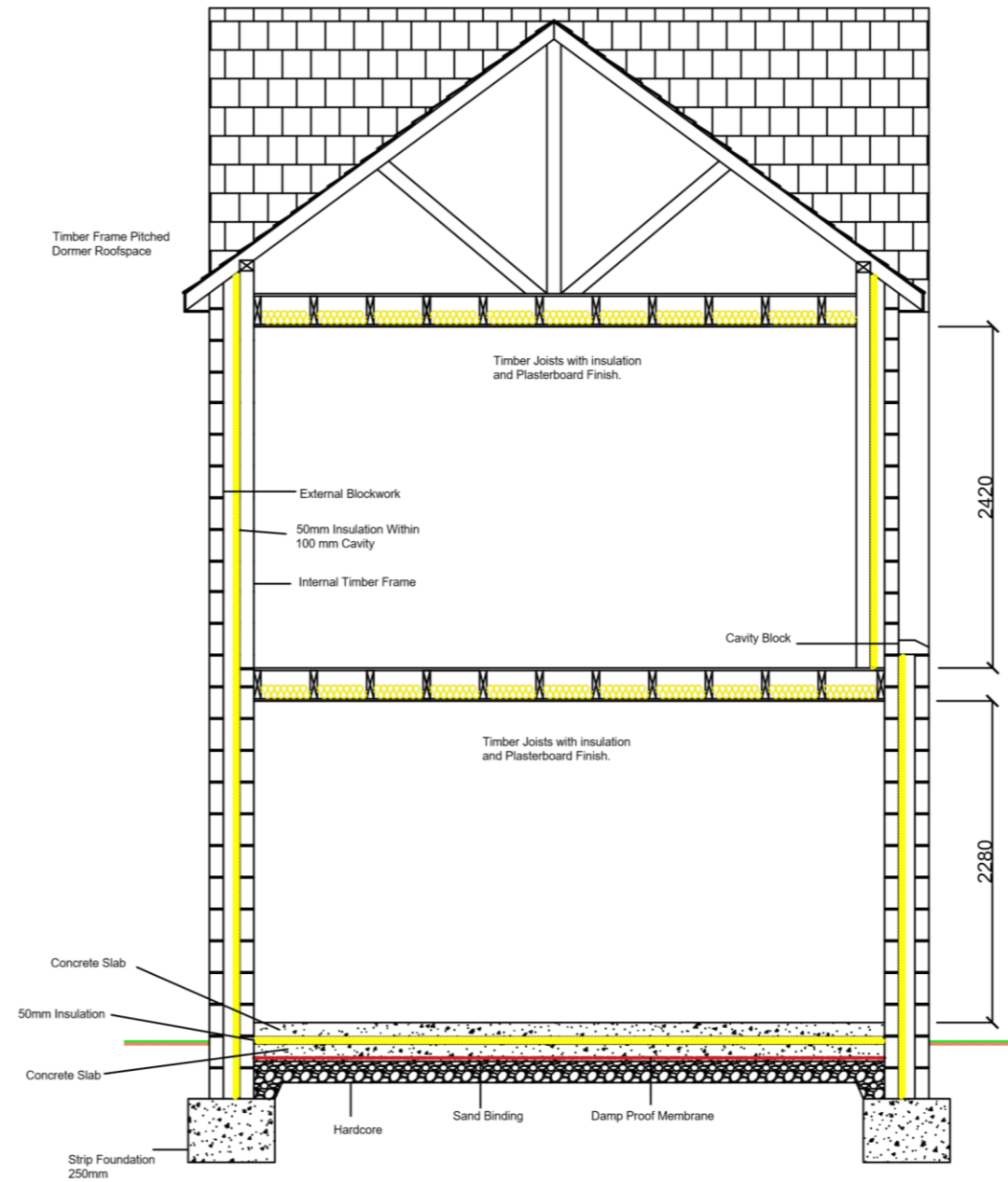
Detailed Section
