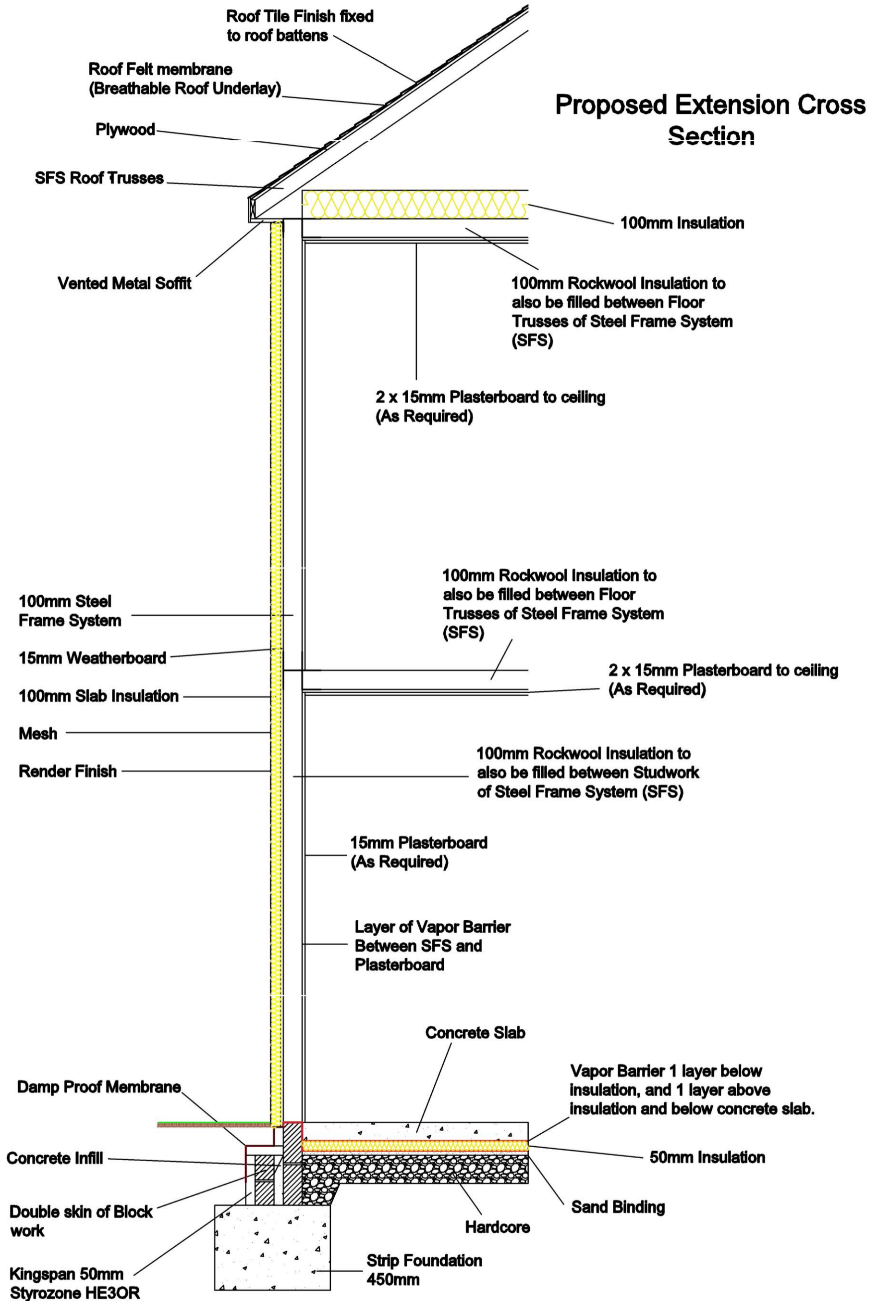
James Reynolds Proposed Extension Scale 1-20 Detailed Section
